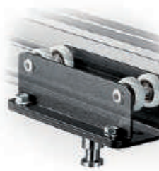
DISMOUNTABLE SLIDING CARRIAGE WITH 4 WHEELS AND 16MM SPIGOT FF3228
